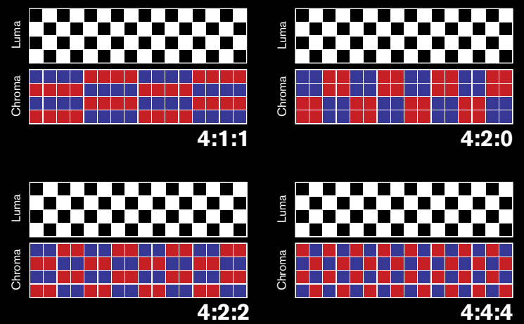
Chroma Subsampling
